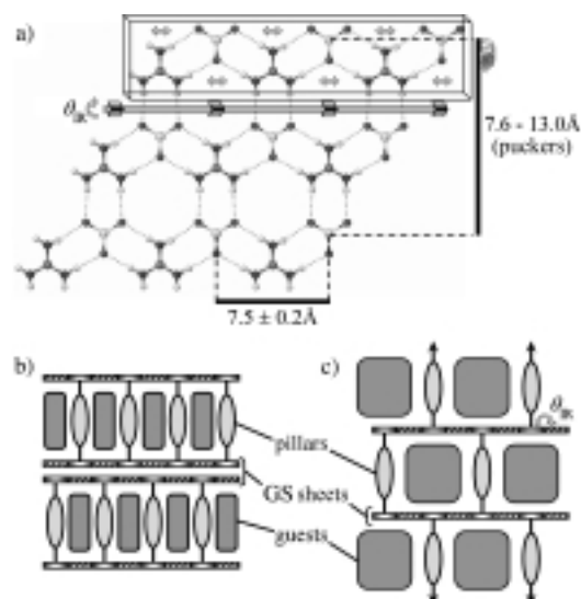
Figure 1. a) The quasihexagonal 2D hydrogen-bonded GS sheet consisting of connected 1D ribbons (boxed) that can pucker by angle \theta_{\text{IR}} . b) Pillared discrete bilayer. c) Pillared continuous “brick” architecture.
